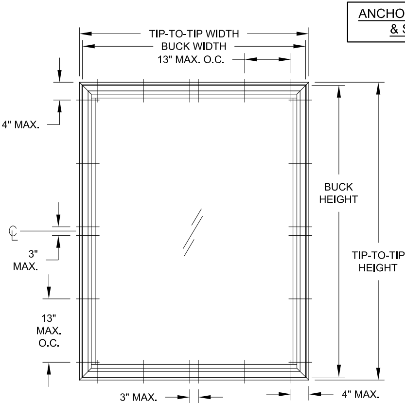
FLANGE/EQUEL-LEG FRAME
