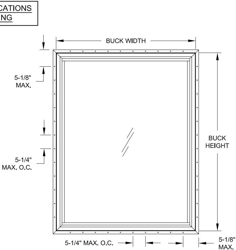
FLANGE FRAME WITH ADD-ON FIN
